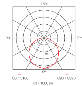
LINE LIT 2000 lm 48" Opal
